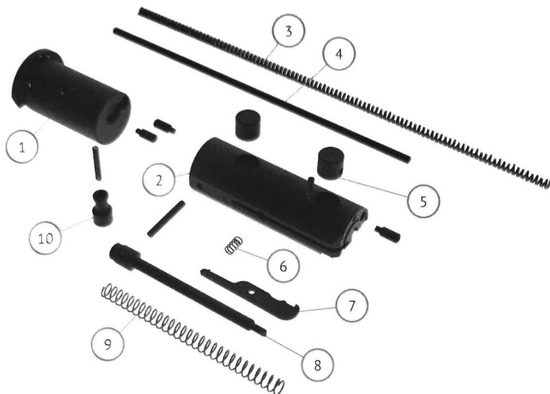
bolt assembly of the interchangeable system
